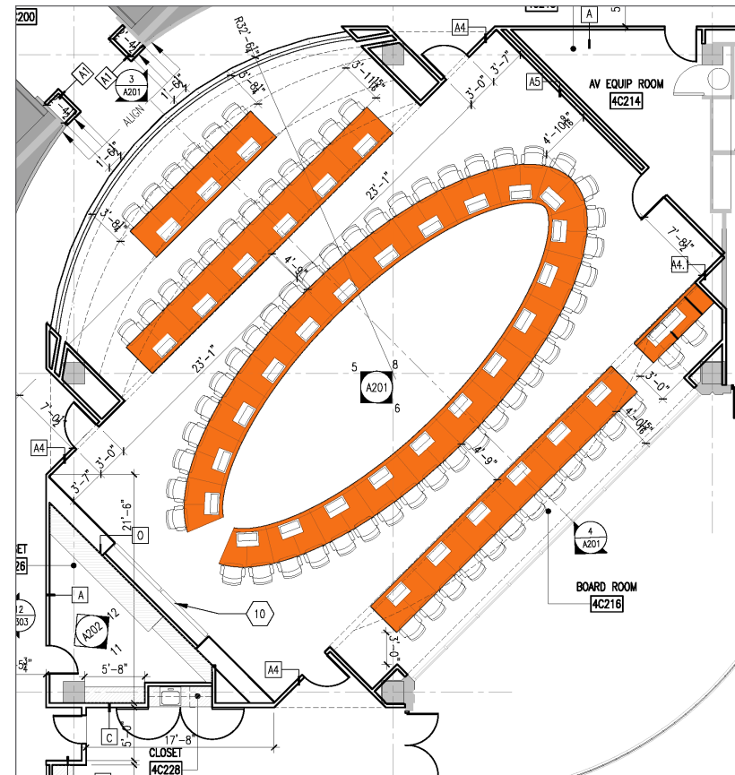
floor plan
